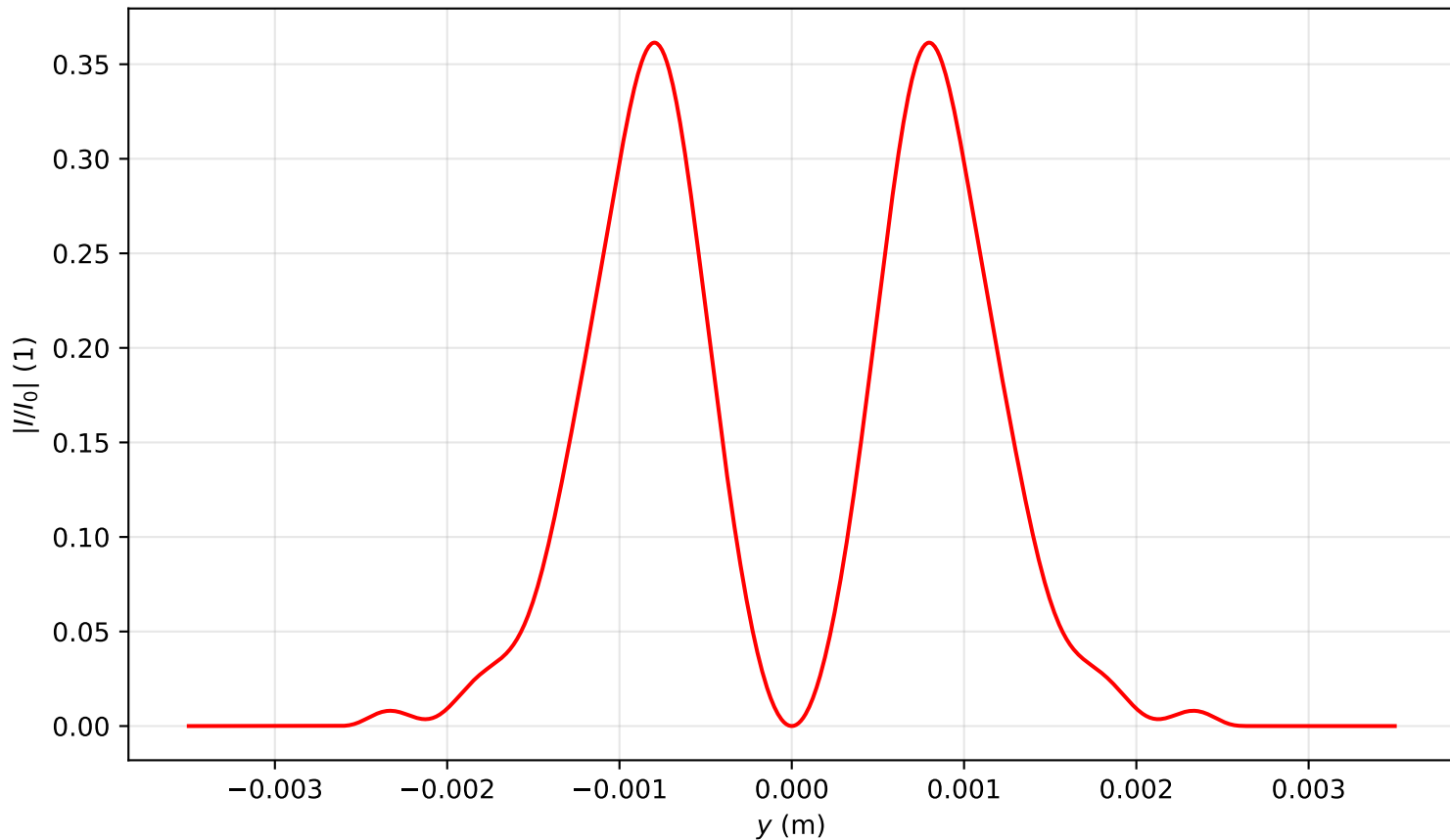
Intensity profile I(x=0, y, z=3.264)/I_0 , \text{Pin}=3.0\text{Pcr} , artificial time
